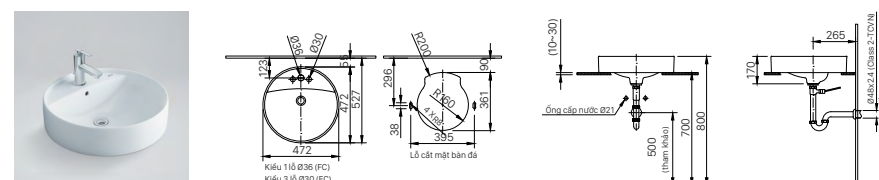
AL-294V (EC/FC) | L-294V (EC/FC)
