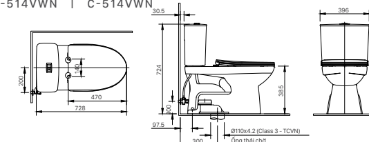
AC-514VAN | C-514VAN | AC-514VWN | C-514VWN
