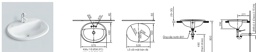
AL-2395V (EC/FC) | L-2395V (EC/FC)
