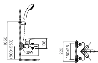
BFV-1403S-4C | BFV-1403S-7C | BFV-1403S-8C | BFV-1403S-3C
